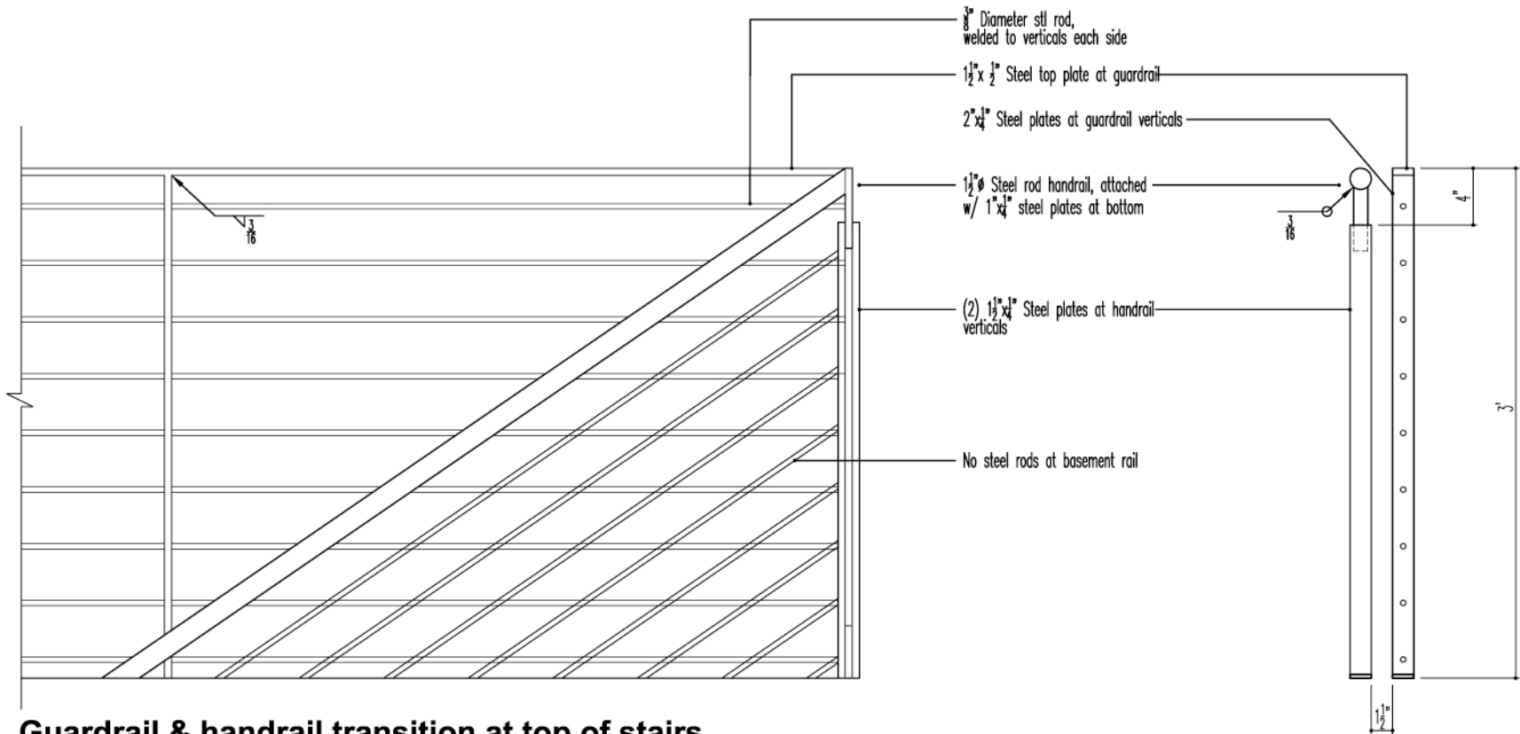
Guardrail & handrail transition at top of stairs
